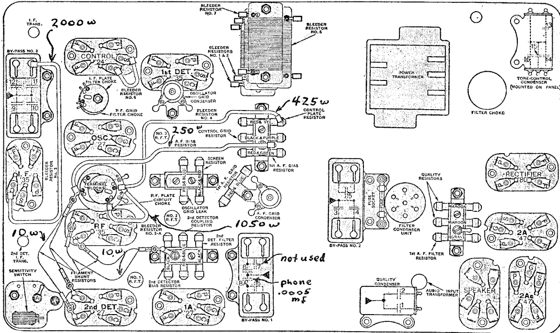
BOTTOM CHART.
